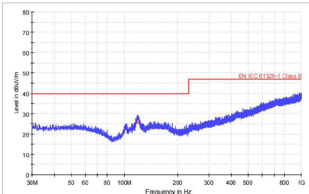
RE_VULB9168_pre_Cont_EN 55032_30-1000
